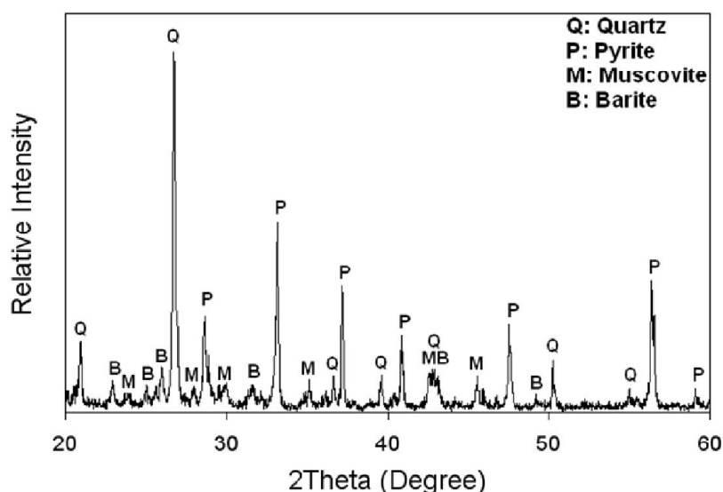
Fig. 1. XRD pattern of the used concentrate.
